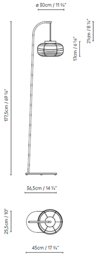
Technical drawing
