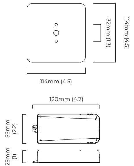
North America junction box cover
